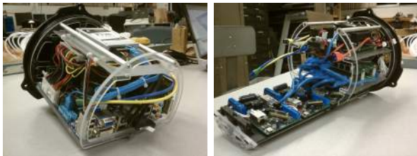
Figure 5: Left: Main pressure vessel forward tray, Right: Main pressure vessel rear tray.
