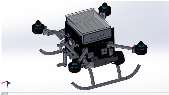
Fig 1. Full model of Cubeception 3.5.
