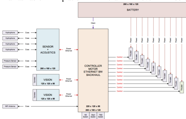
Fig 2. High level overview of Cubeception 3.5’s hardware.
