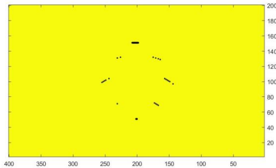
Fig 13. Three hydrophone array detecting eight objects placed in an approximately circular fashion using time tables.
