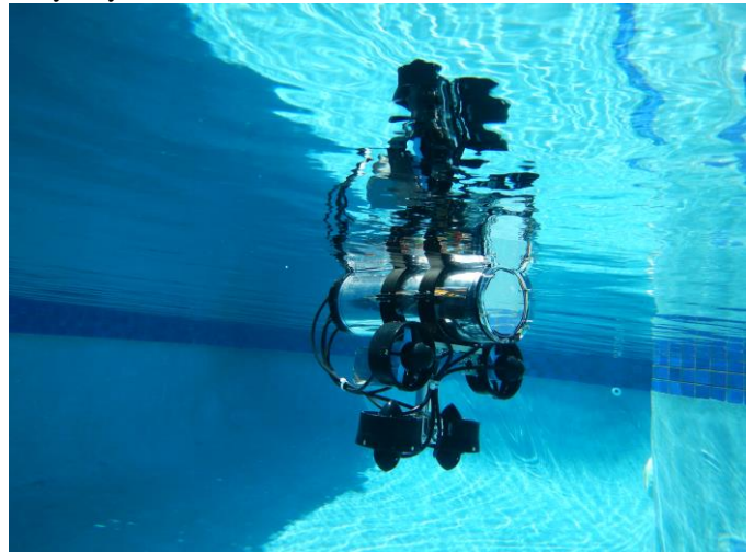
Fig 9. Minisub mechanical layout.
