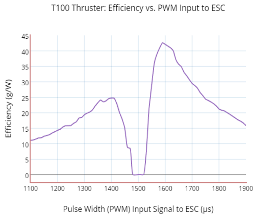
Fig 10. Thruster efficiency of T100.
