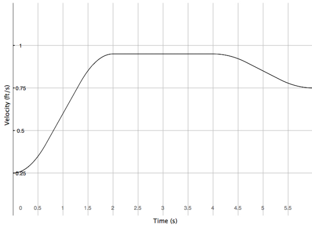
Fig 8. Another velocity over time curve for a motion profile.
