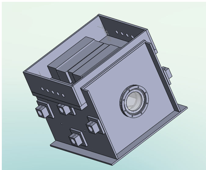
Fig 4. Cube core with integrated battery box on top.
