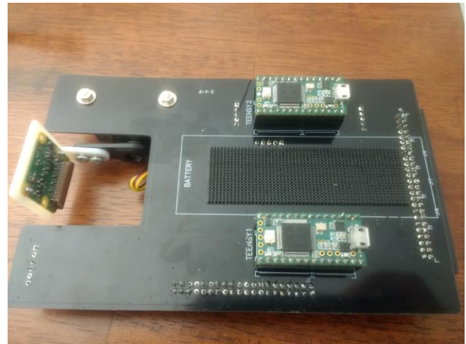
Fig 11. Custom PCB for minisub.
