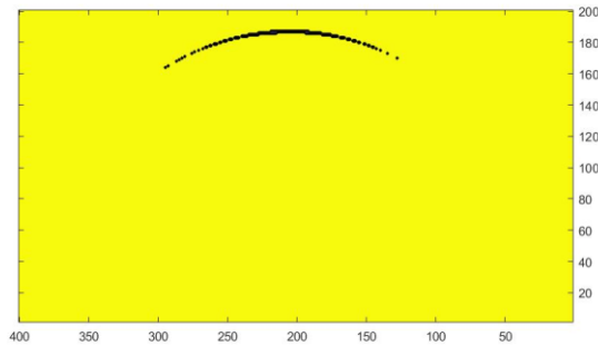
Fig 12. Two hydrophone array comparing received times to a time table generated based on expected times. The black curve represents possible locations.
