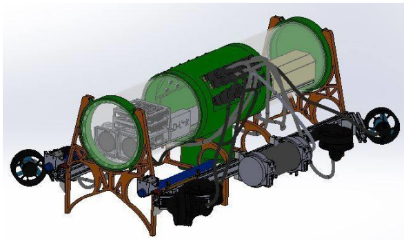
Fig. 1. Zeabus platform
