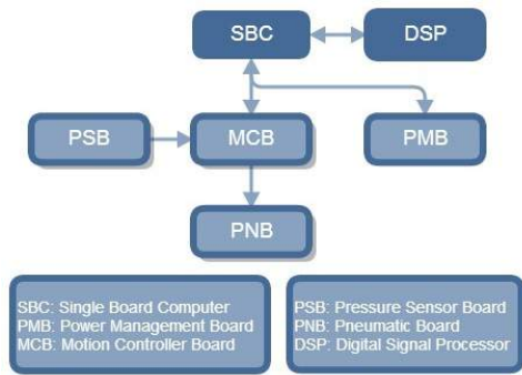
Figure 14: Inter Board Communication
