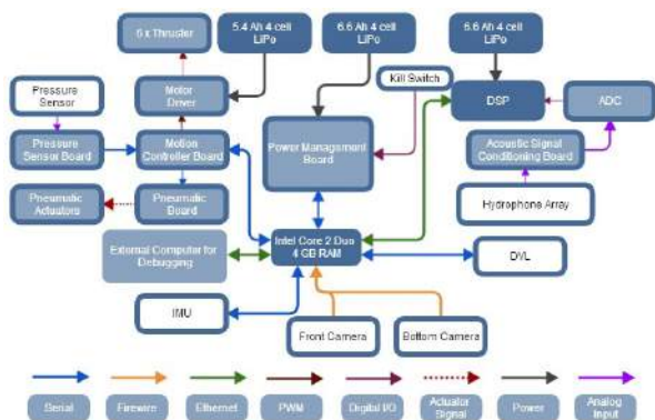
Figure 6: Electronics System Communication Diagram
