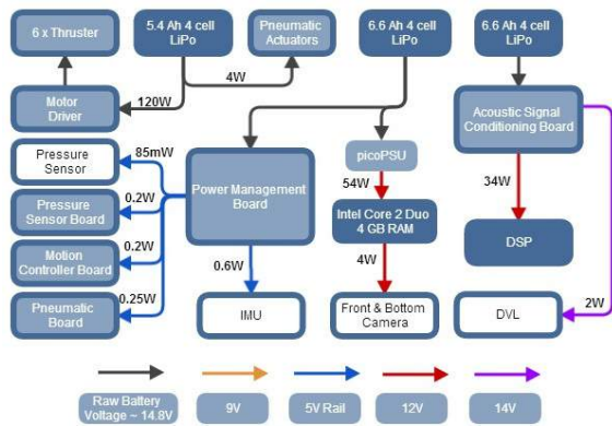
Figure 8: Power Distribution Diagram
