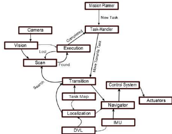
Figure 16: Software Control Flow
