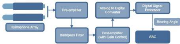
Figure 10: Acoustic Localization: Five stage process
