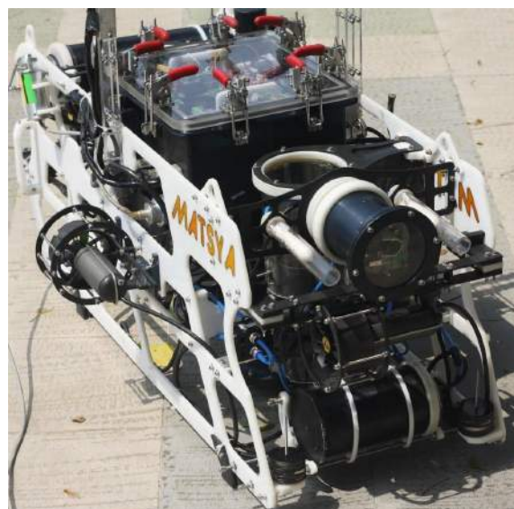
Figure 1: Matsya 3.0
