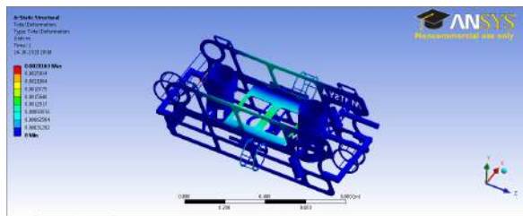
Figure 4: Frame analysis in ANSYS
